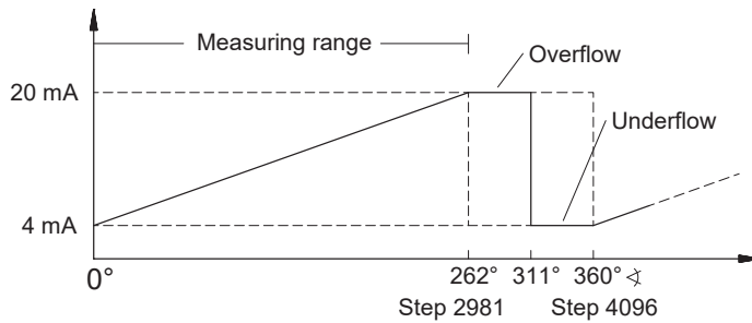
Characteristic curve: measuring angle 262° as an example
